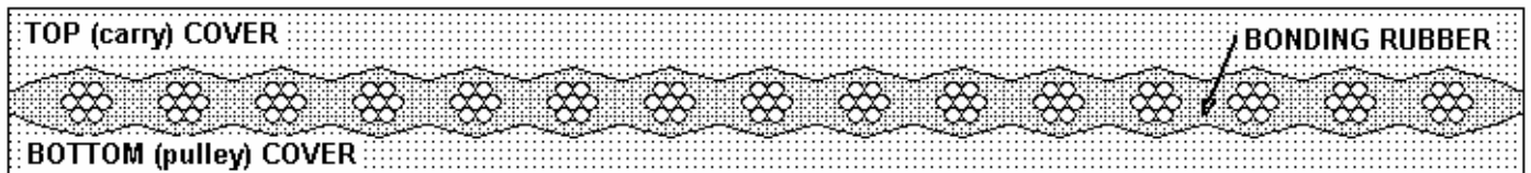
FIG. 1 BELT CONSTRUCTION
